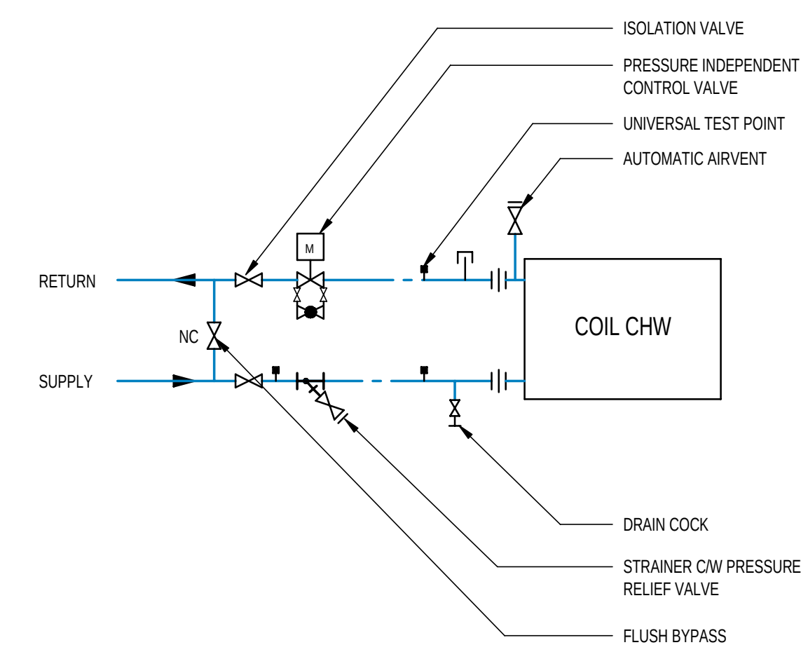
DETAIL A - CHW COIL CONNECTION DETAIL N.T.S.
